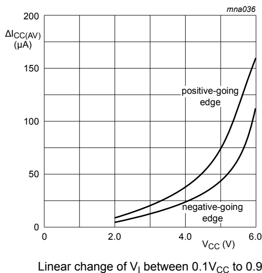
Fig. 15. Average additional I_{\text{CC}} for 74AHC3G14 Schmitt trigger devices
