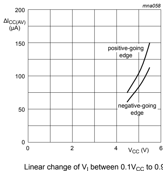
Fig. 16. Average additional I_{\text{CC}} for 74AHCT3G14 Schmitt trigger devices
